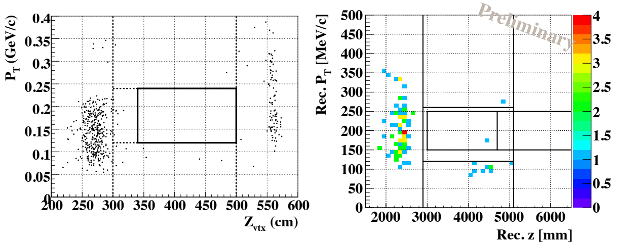
Figure 7.1.1: The scatter plot of the decay position of the reconstructed \pi^0 on the K_L beam versus the transverse momentum of the \pi^0 for the result of E391a (left) [4] and that for KOTO (right) [42]. Black square in the left plot shows the allowed region of the signal in E391a. Inner most black square in the right plot shows the signal region in the first physics run. Dotted lines in the left plot and other black lines in the right plot indicate boundaries to classify events for the background study.
