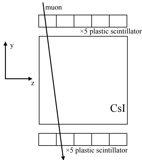
Figure 2.3.4: Plastic scintillators used in the energy calibration of the calorimeter.
